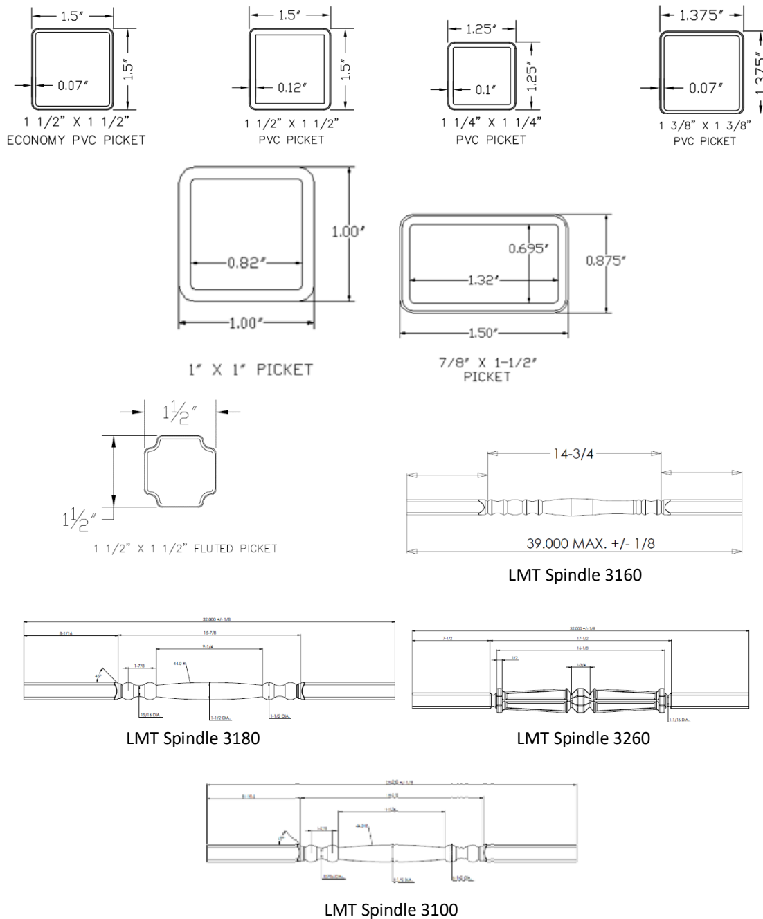
FIGURE 3 – PVC BALUSTERS
